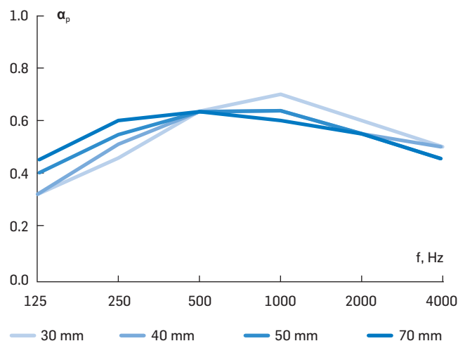
Suspension 200 mm
