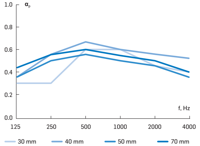
Suspension 200 mm
